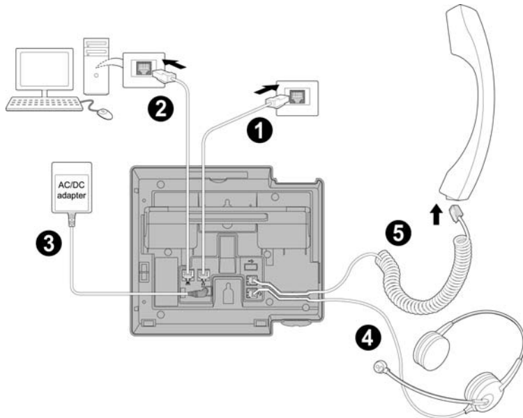
Figure 2: Phone connections
