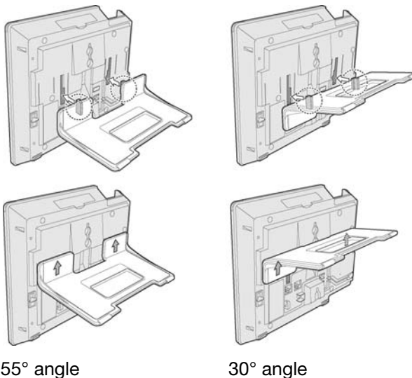
Figure 3: Installing the foot stand
